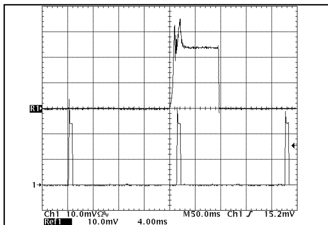
Figure 18: Load current ( 10\ \text{A}/\text{div} ) as a function of time when the converter attempts to turn on into a 10\ \text{m}\Omega short circuit. Top trace ( 4.0\ \text{ms}/\text{div} ) is an expansion of the on-time portion of the bottom trace.
