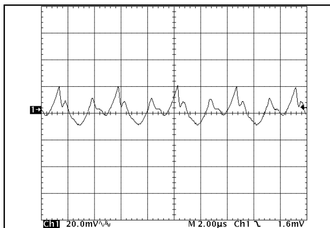
Figure 16: Output Voltage Ripple at nominal input voltage and rated load current ( 20\ \text{mV}/\text{div} ). Load capacitance: 1\ \mu\text{F} ceramic capacitor and 10\ \mu\text{F} tantalum capacitor. Bandwidth: 20\ \text{MHz} . See Figure 13.
